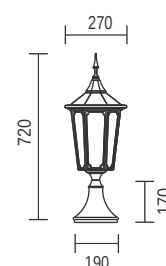
T108D - Pedestal
