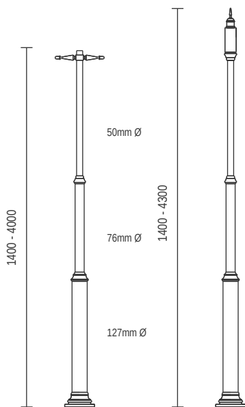
P107 - Heavy Post Single
