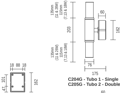
Back Plate Detail
