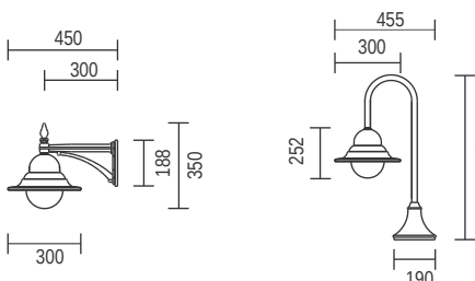
T114B - Wall Bracket
