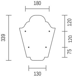
Back Plate Detail
