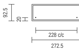
Back Plate Detail
