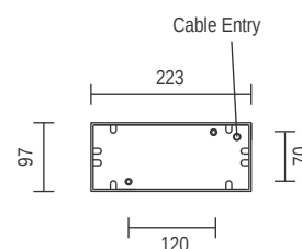
Serengeti Back Plate Detail
