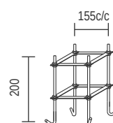
A130 - Standard Post Bolt Cage
