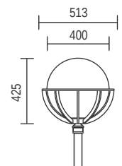
T129A - 400mm 8 Arm Basket Post Top
