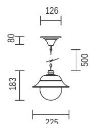
T113E - Chain Hanging
