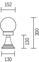
T111D - Pedestal 6 inch bowl
