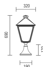
T107D - Pedestal
