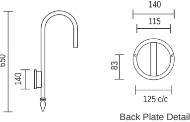
A156 - Gooseneck Wall Bracket
