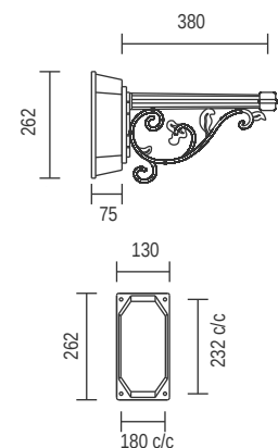
A159 - Large bracket block with filigree bracket
