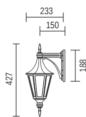
T105B - Down Facing
