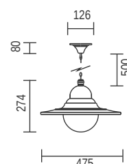
T116E - Chain Hanging
