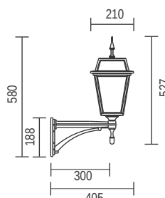
T109C - Up Facing
