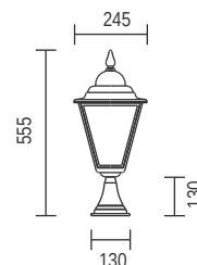
T121D - Pedestal
