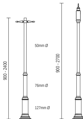
P108 - Standard Post Single
