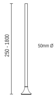
P112 - Column
