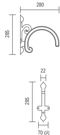
A158 - Classic Wall Bracket
