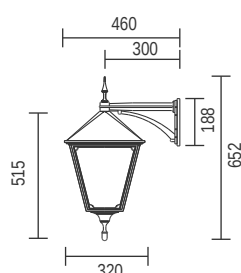
T107B - Down Facing
