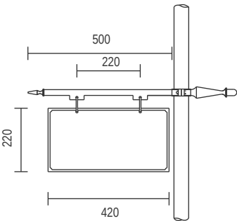
A121 - Clamp on sign arm complete with board A122 - Clamp on sign arm only. (51mm pole or 76mm pole)
