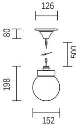
T111E - Chain Hanging 6 inch bowl
