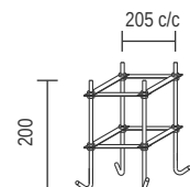
A164 - Bolt Cage
