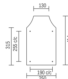
Empire Back Plate Detail
