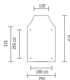
Back Plate Detail
