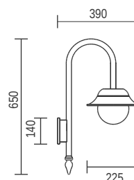
T135B - Gooseneck Bracket
