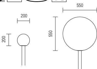
T132Z - 250mm Sphere
