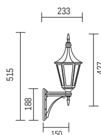
T105C - Up Facing
