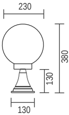
T112D - Pedestal 8 inch bowl
