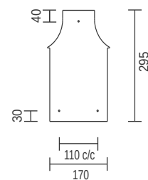
Back Plate Detail
