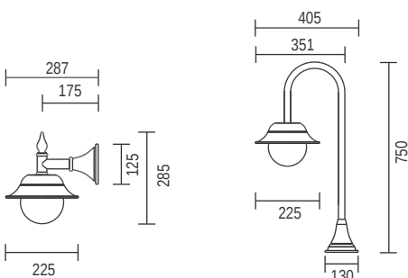
T113B - Wall Bracket
