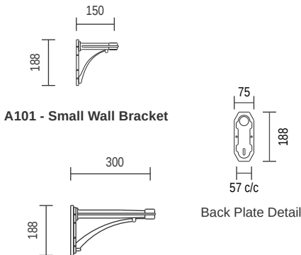
A102 - Large Wall Bracket
