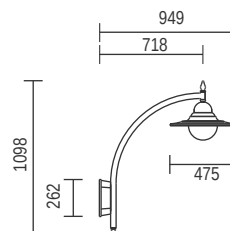
T136B - Curved Wall Bracket
