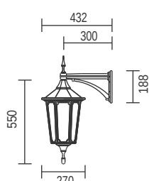
T108B - Down Facing
