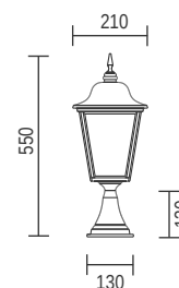
T106D - Pedestal
