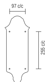
Back Plate Detail
