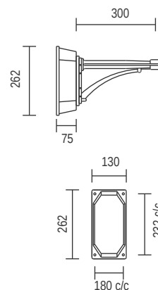
A120 - Large bracket block PL9W to PL26W, 80W MV to 125MV, or 70W HPS gear
