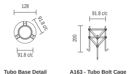
Tubo Base Detail
