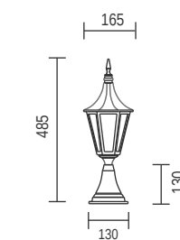
T105D - Pedestal
