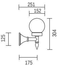
T111C - Standard Bracket 6 inch bowl
