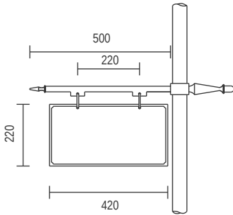
A123 - Slide on sign arm complete with board A124 - Slide on sign arm no board (51mm pole only)
