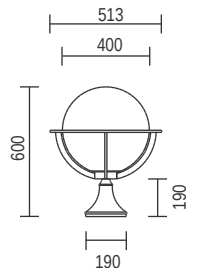
T128D - 400mm 4 Arm Basket Pedestal
