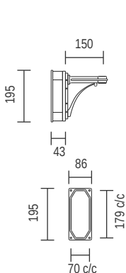
A119 - Small bracket block PL9W to PL26W gear
