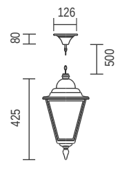
T121E - Chain Hanging
