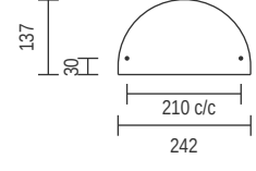
Back Plate Detail
