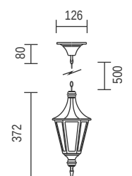
T105E - Chain Hanging
