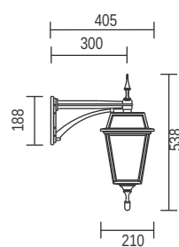
T109B - Down Facing
