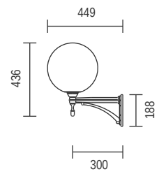
T126C - 300mm Sphere Wall Bracket
