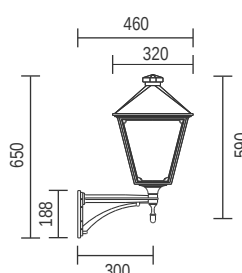
T107C - Up Facing
