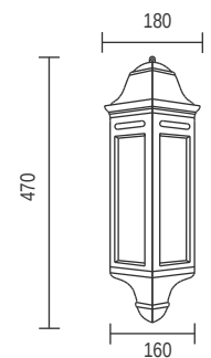
Front View
