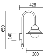
T137B - Gooseneck Bracket
