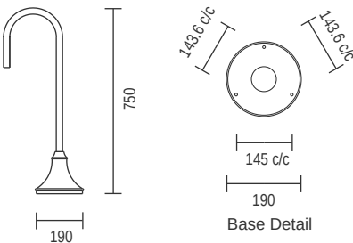
A155 - Gooseneck Pedestal
