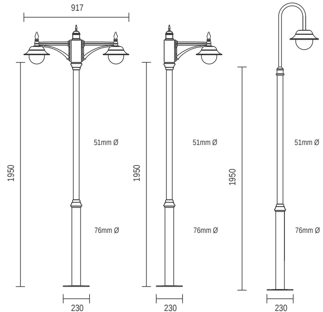
T1131 Basic Double Post
