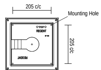
Back Plate Detail
