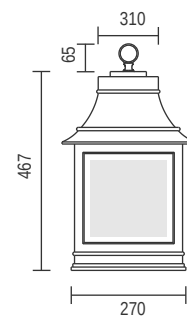
Empire Front View
