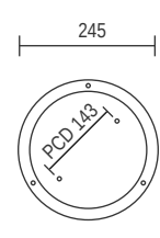
Back Plate Detail
