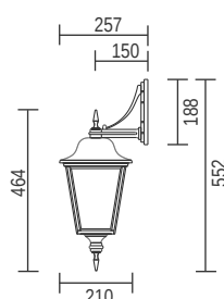
T106B - Down Facing
