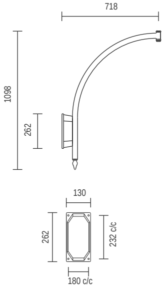
A154 - Curved Wall Bracket
