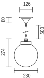
T112E - Chain Hanging 8 inch bowl
