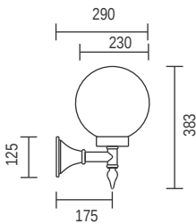
T112C - Standard Bracket 8 inch bowl
