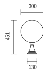
T126D - 300mm Sphere Pedestal
