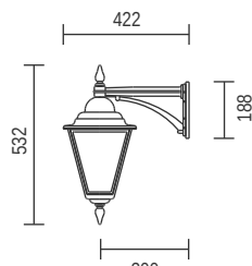
T121B - Down Facing
