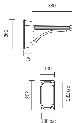
A162 - Large bracket block with extra large bracket
