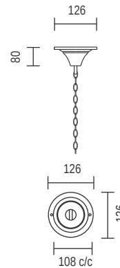
A157 - Ceiling Bracket with chain
