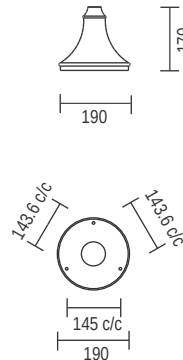
A108 - Large Pedestal
