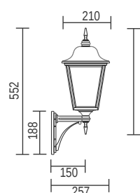
T106C - Up Facing
