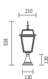
T109D - Pedestal
