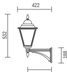
T121C - Up Facing
