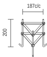
A132 - Heavy Post Bolt Cage
