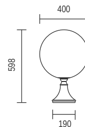
T131D - 400mm Sphere Pedestal
