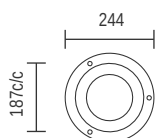
P107 - Heavy Post Single
