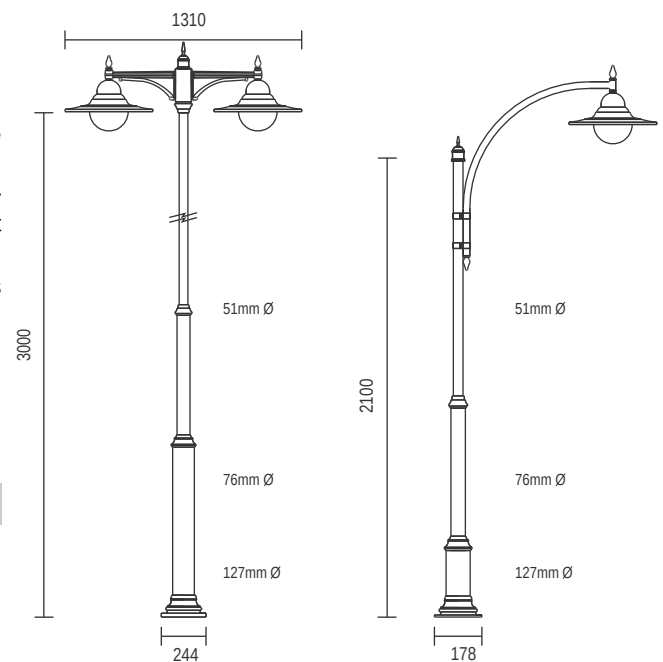
P107 - Heavy Post P1167 - Double Large Rexford Bracket
