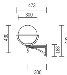
T123C - 300mm 2 Arm Basket Wall Bracket
