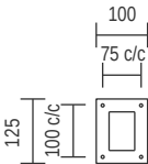
A147 - Mounting plate accessory
